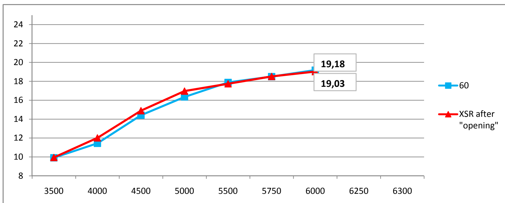
MAXIMUM FUEL CONSUMPTION (l/h)
