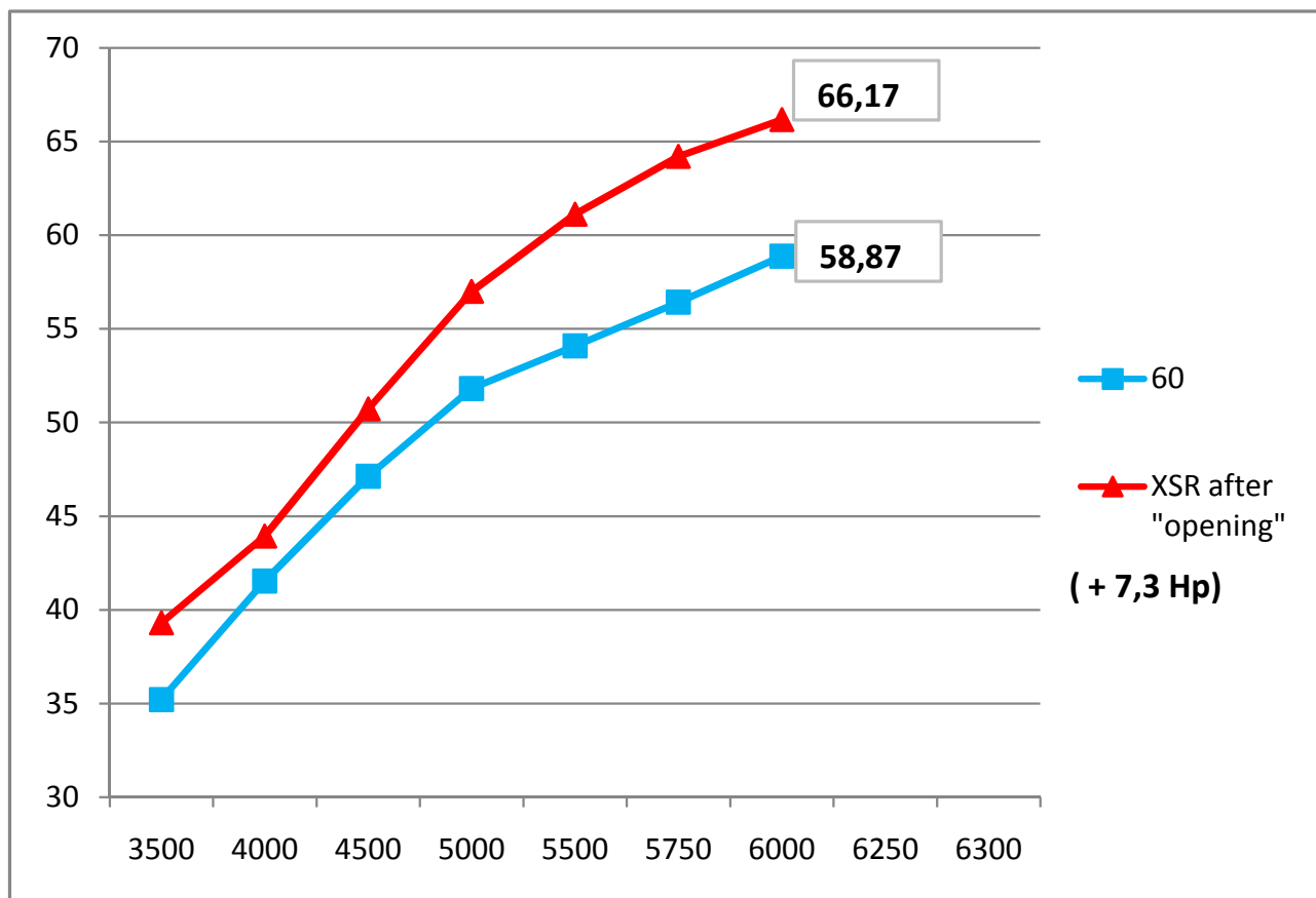
POWER AT THE PROPELLER SHAFT (HP)
