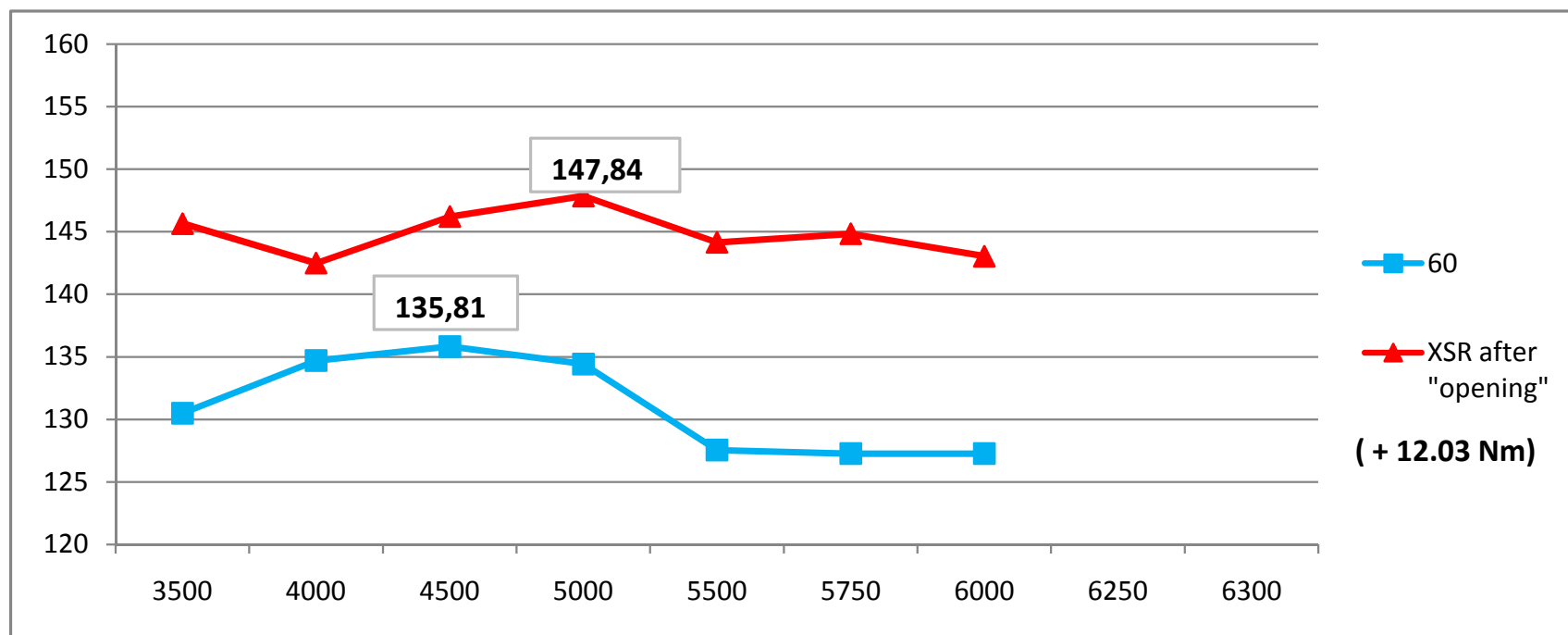
TORQUE AT THE PROPELLER SHAFT (Nm)
